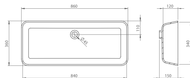
ICE XL ugradbeni built-in
