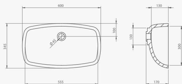
STYLE ugradbeni built-in
