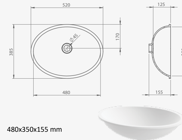
ELIPSO ugradbeni built-in
