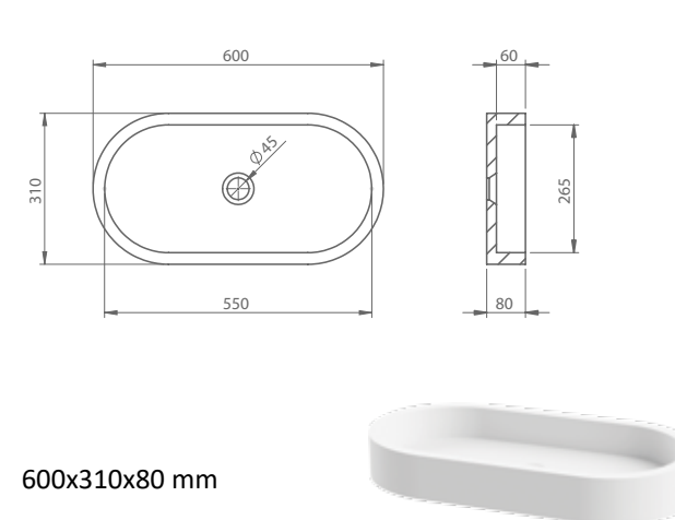
OVAL 60 ugradbeni built-in ugradnja na pult installation on a table top
