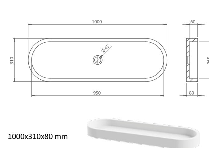
OVAL 100 ugradbeni built-in ugradnja na pult installation on a table top
