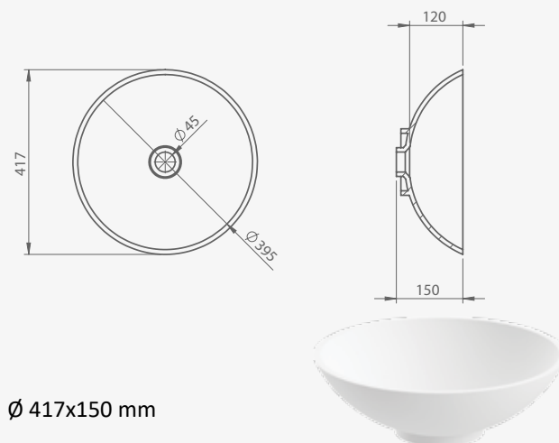
FI 40 ugradbeni built-in ugradnja na pult installation on a table top
