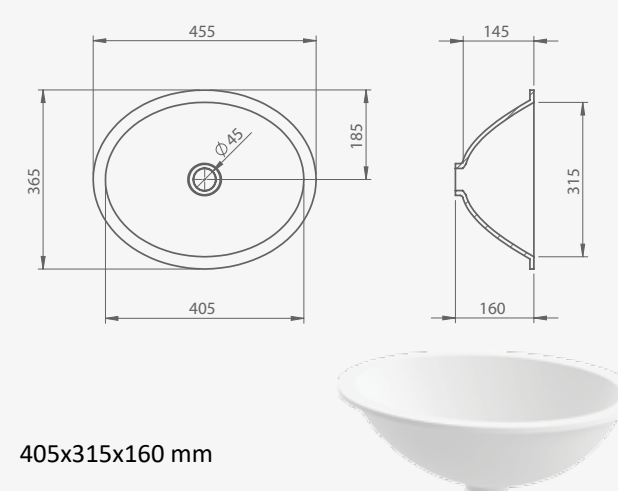
ELIPSO SMALL ugradbeni built-in
