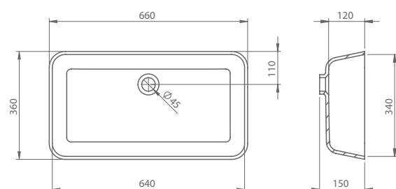
ICE ugradbeni built-in
