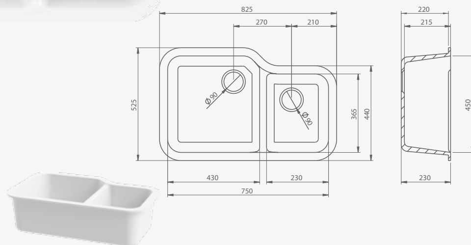
DVODJELNI R/L ugradbeni built-in nadgradbeni semi built-in
