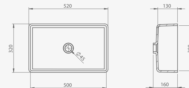
CLARION ugradbeni built-in
