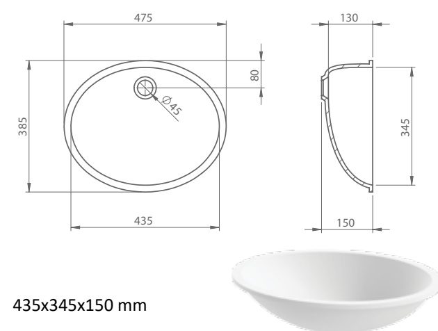
EURO ugradbeni built-in
