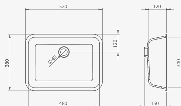
ICE SMALL ugradbeni built-in
